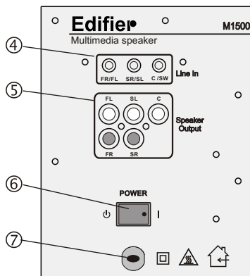
Back Panel
